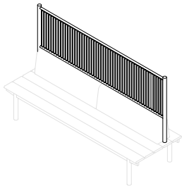
Dowel Partition Only for Configurations 2.5, 7.5
